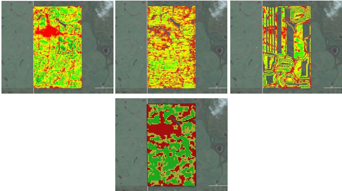
Figure 3. Calculation of low, average and high production zones from 2011, 2012, and 2013 yield monitor data for the SK1 field.
